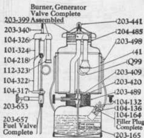
For Model No. L327 Quick-Lite Lanterns (With Separate Pump)
