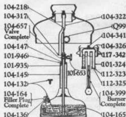
For Model "C" Quick-Lite Lamps (With Separate Pump)
