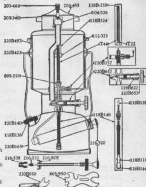
For Models Nos. 220B and 228B
