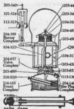
For Models No. L427 (1927) and L227 Lanterns (With Fully Concealed Built-in Pump)
